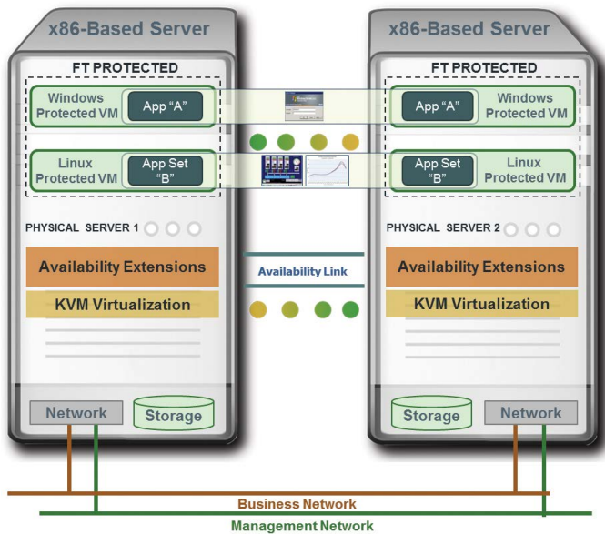
Stratus everRun Enterprise Architecture Diagram
